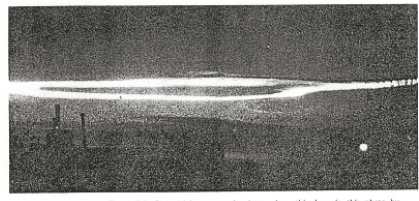
The ring-cloud over Flagstaff is flattened by perspective into a long thin loop in this photo by Lynne E. Cobble, taken at Albuquerque, N. M., some 240 miles from the cloud. Intense low-angle forward-scattering by the cloud particles (assumed to be water or ice) creates strong contrast against the twilight sky. Sun had set at Albuquerque almost a half hour before this photo was made at 1840 MST. Kodak Retina Reflex camera F4 1/8th of sec. with 135mm telephoto lens. Photo courtesy Sgt. Arthur A. Francis, Kirland AFB, who is making a study of the phenomenon.
